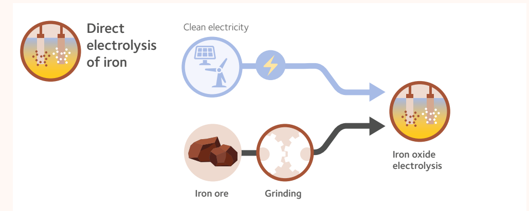
Figure X : Direct electrolysis route
