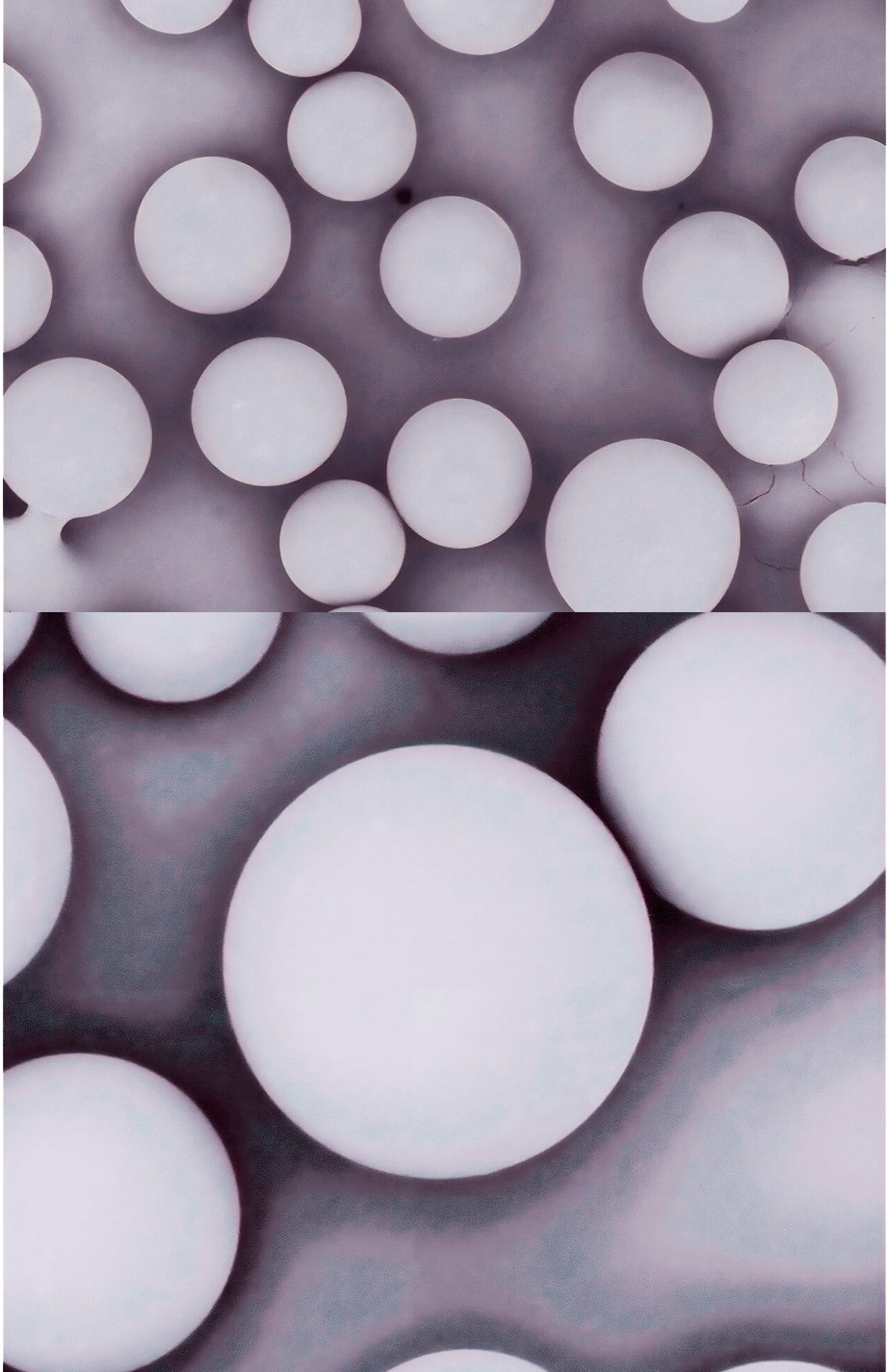
SEM images of a powder spheroidized in AlphaPowders process, AlphaPowders
