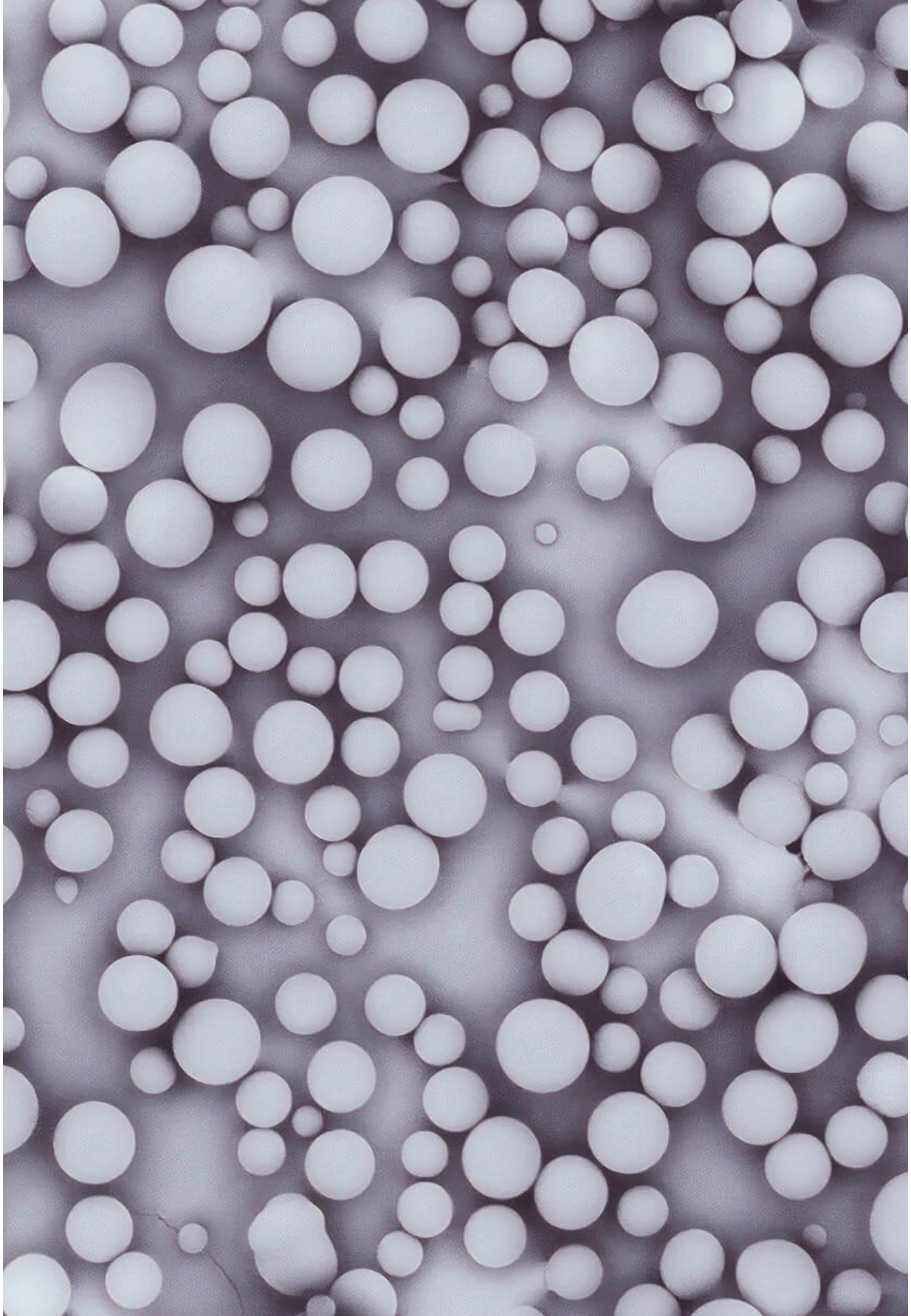
SEM image of a powder spheroidized in AlphaPowders process, AlphaPowders
