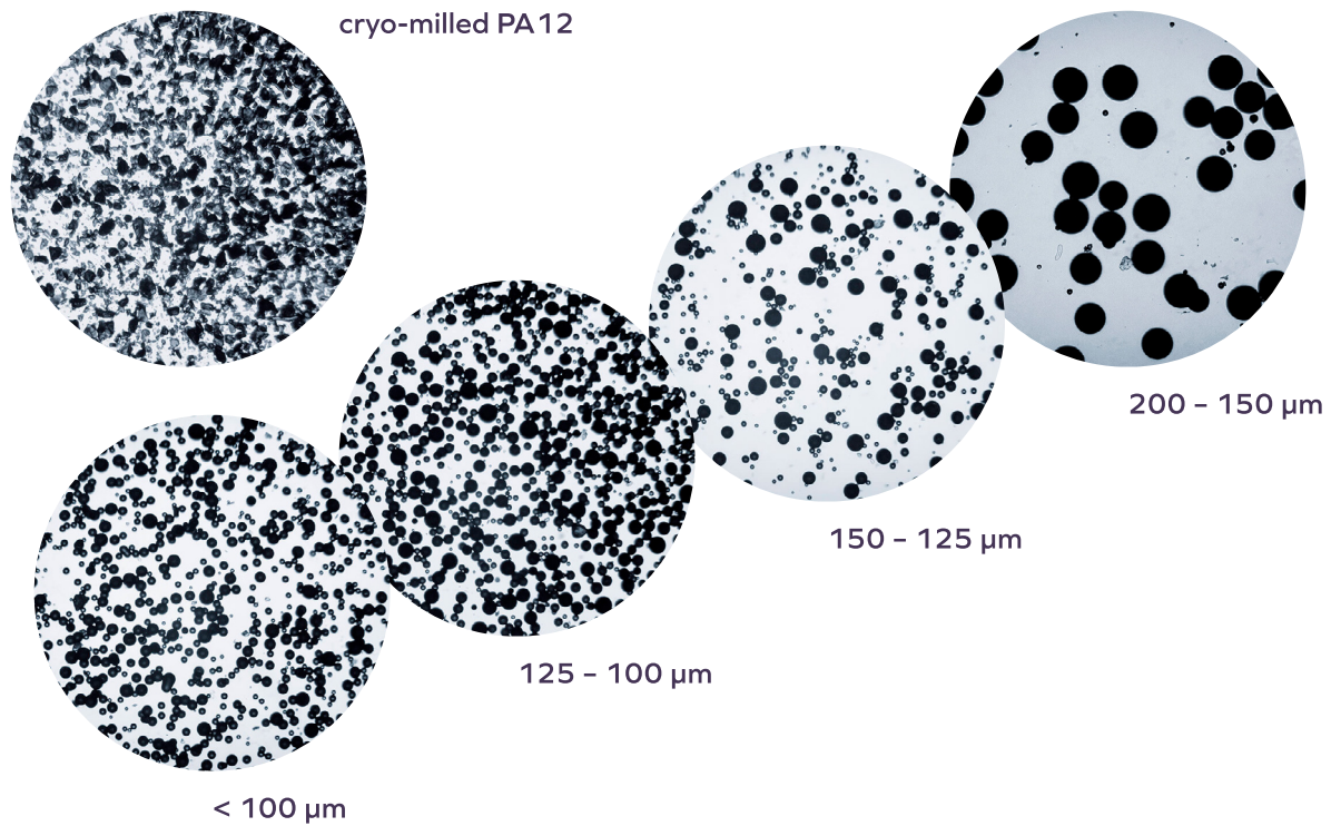
Spheroidization can be tuned to work on every size fraction. Visible light microscope images, AlphaPowders
