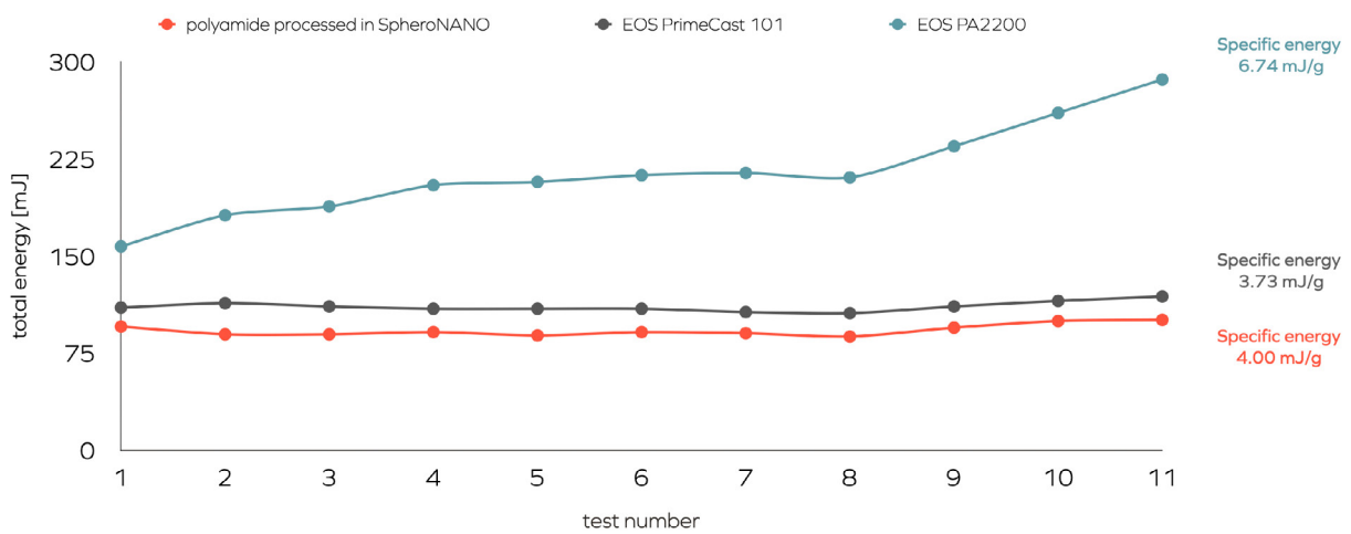
Cryo-milled and spheroidized PA12 has excellent flow properties. FT4 measurements courtesy of Wrocław University of
