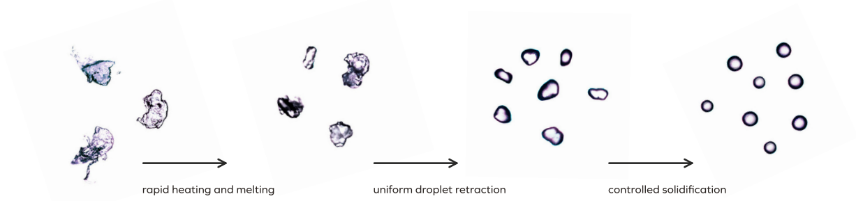
Spheroidization mechanism, AlphaPowders
